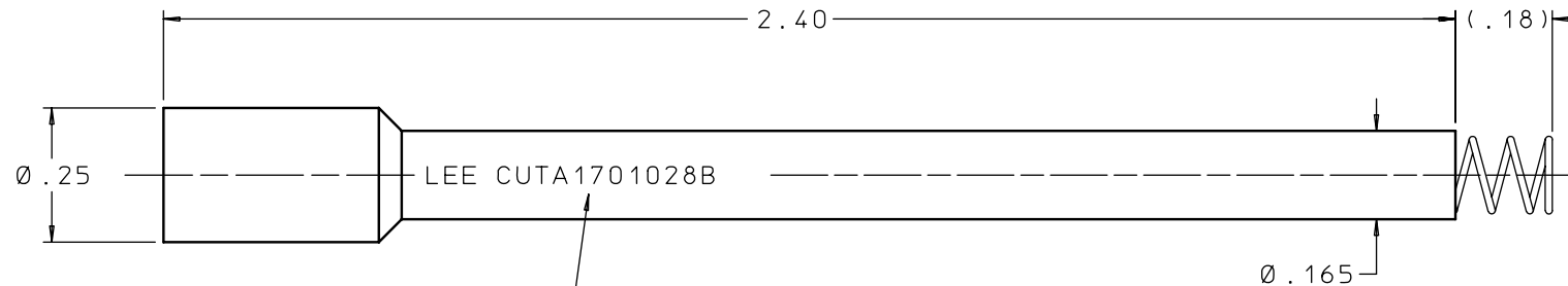
SCREEN EXTRACTION TOOL
