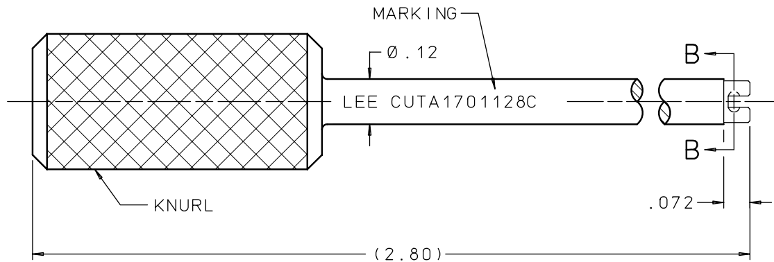
SPRING INSTALLATION/EXTRACTION TOOL
