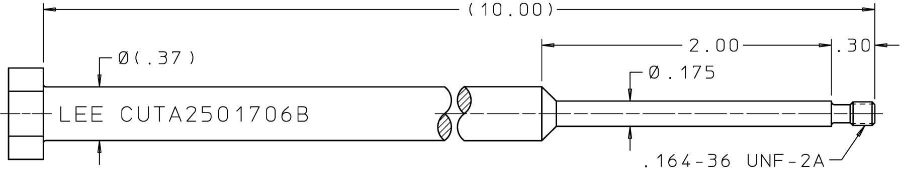
BODY & PIN EXTRACTION TOOL
