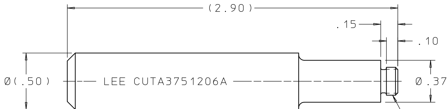
PIN INSTALLATION TOOL
