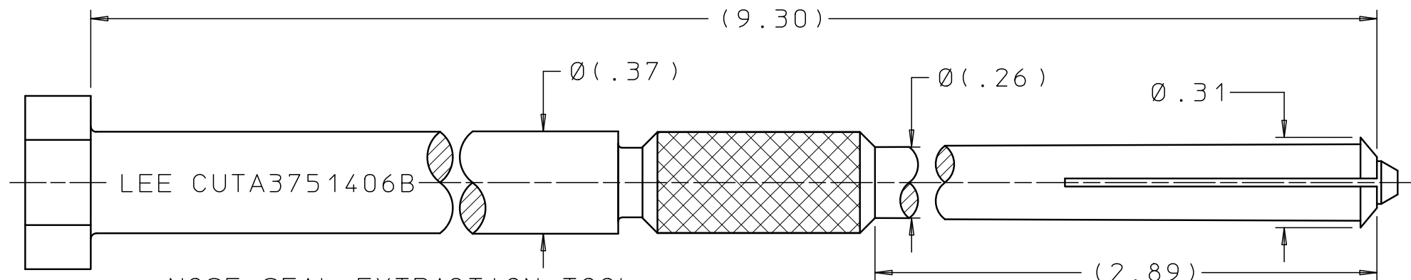
NOSE SEAL EXTRACTION TOOL
