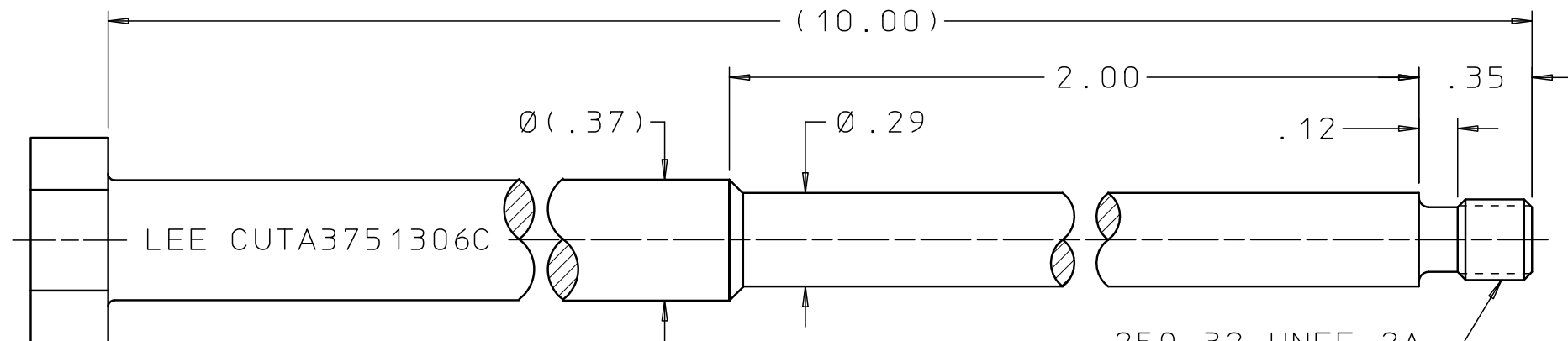
BODY INSTALLATION & EXTRACTION TOOL PIN EXTRACTION TOOL
