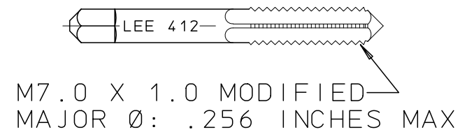
STARTER TAP PLUG EXTRACTION CUTM4125503B
