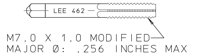
BOTTOMING TAP PLUG EXTRACTION CUTM4625503B
