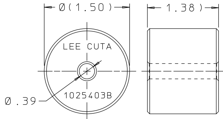
STRIKER, PLUG
