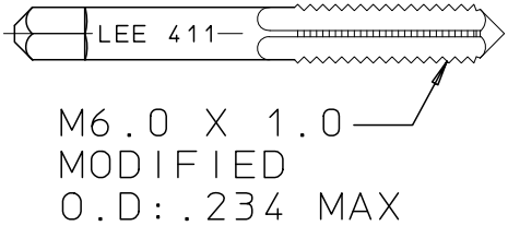
STARTER TAP PIN EXTRACTION CUTM4115403B
