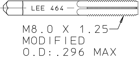
BOTTOMING TAP PLUG EXTRACTION CUTM4645503B
