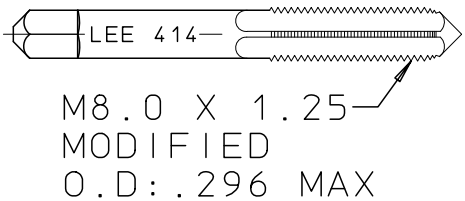
STARTER TAP PLUG EXTRACTION CUTM4145503B
