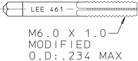
BOTTOMING TAP PIN EXTRACTION CUTM4615403B
