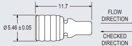
CHECK VALVE
