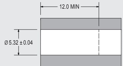
INSTALLATION HOLE
