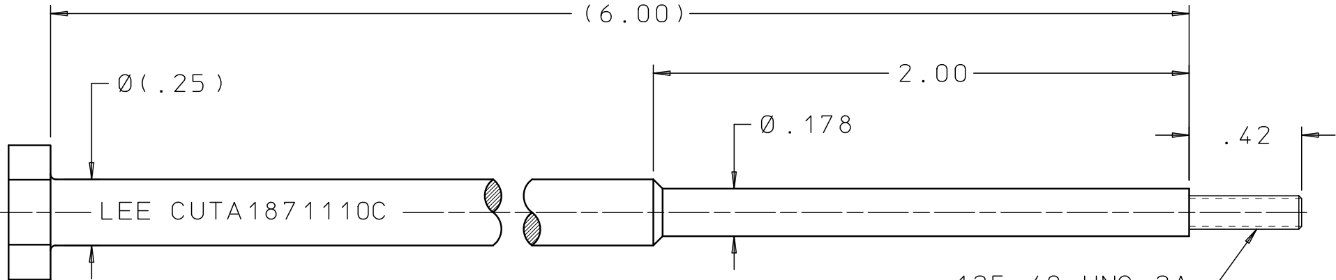
BODY INSTALLATION & EXTRACTION TOOL
