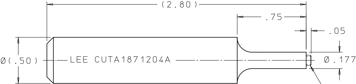
PIN INSTALLATION TOOL
