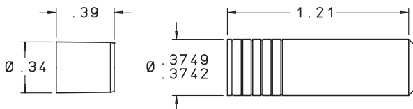
PIN
