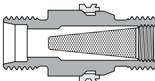
FLARELESS TUBE
