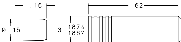
PIN
