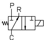
NORMALLY CLOSED
