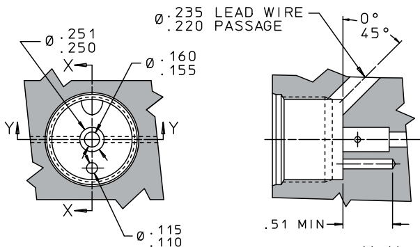
SECTION X-X
