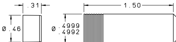
PIN
