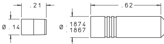
PIN
