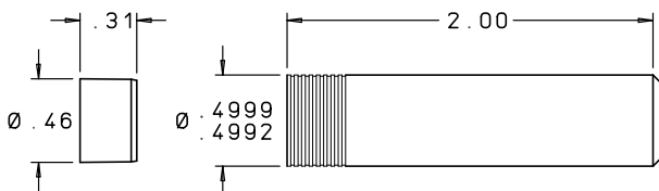
PIN
