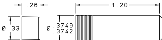
PIN
