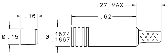
PIN
