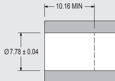
INSTALLATION HOLE
