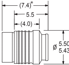
DIMENSIONAL VIEW
