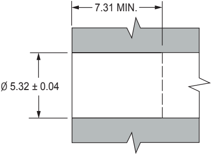
INSTALLATION HOLE
