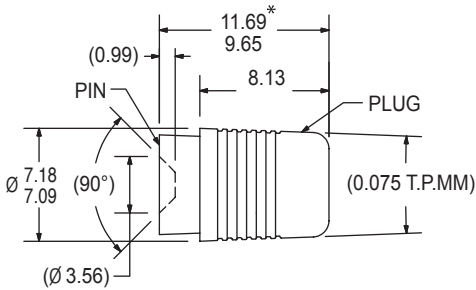
DIMENSIONAL VIEW
