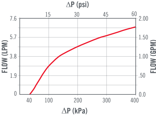
FLOW CURVE FOR 40 kPa VALVE
