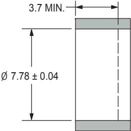
INSTALLATION HOLE
