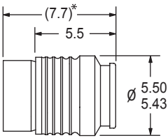
DIMENSIONAL VIEW
