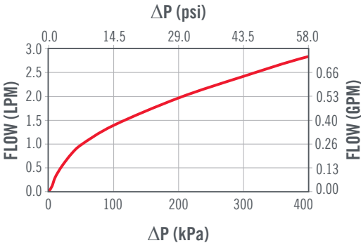
FLOW CURVE FOR 0 kPa VALVE
