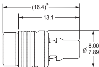
DIMENSIONAL VIEW
