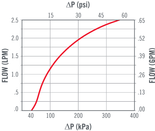
FLOW CURVE FOR 40 kPa VALVE
