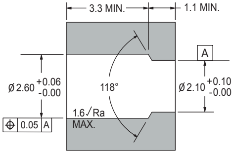
INSTALLATION HOLE
