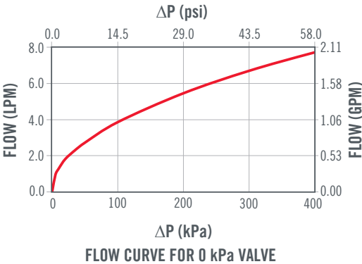
FLOW CURVE FOR 0 kPa VALVE
