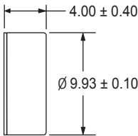
DIMENSIONAL VIEW
