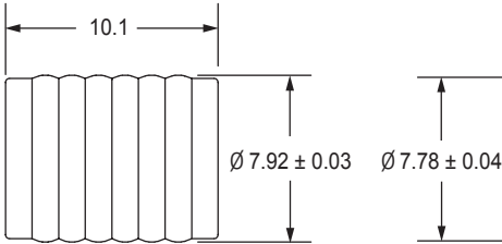
DIMENSIONAL VIEW
