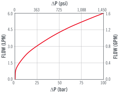
FLOW CURVE FROM PILOTED PORT A TO C, FOR 250 kPa VALVE
