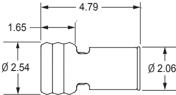
DIMENSIONAL VIEW
