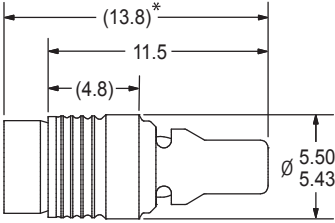
DIMENSIONAL VIEW
