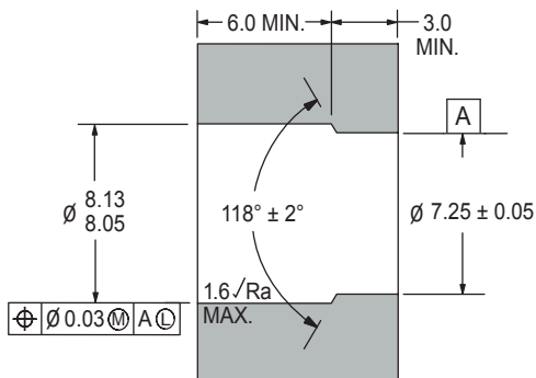
INSTALLATION HOLE
