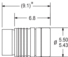
DIMENSIONAL VIEW
