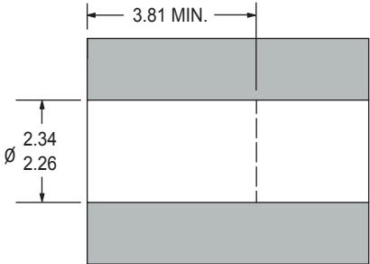
INSTALLATION HOLE
