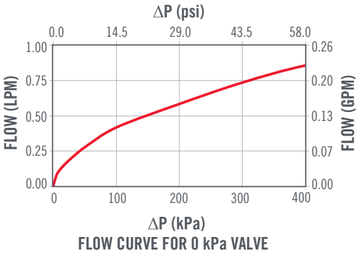
FLOW CURVE FOR 0 kPa VALVE
