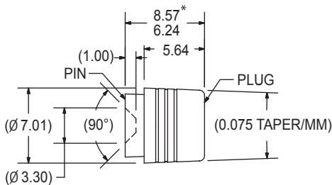
DIMENSIONAL VIEW
