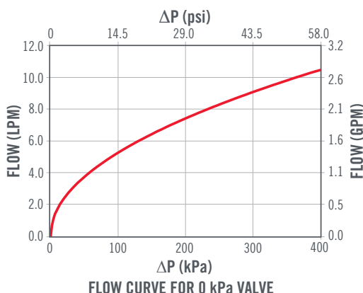
FLOW CURVE FOR 0 kPa VALVE
