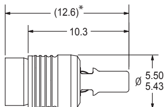
DIMENSIONAL VIEW
