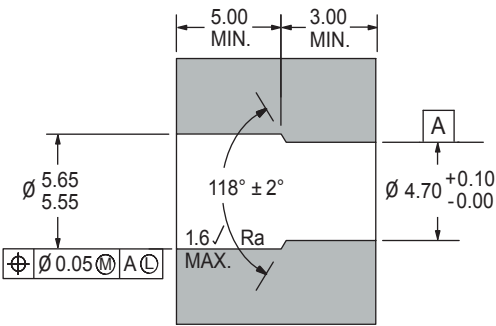
INSTALLATION HOLE
