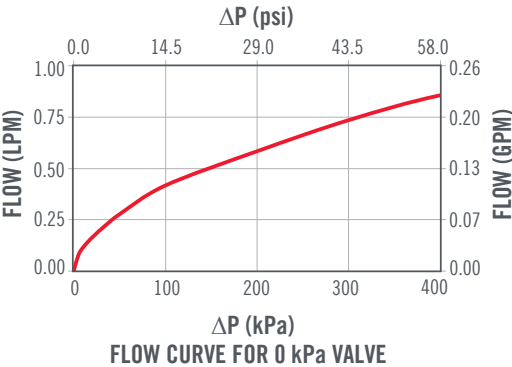
\Delta P vs. FLOW ON WATER AT 27°C (80°F)
