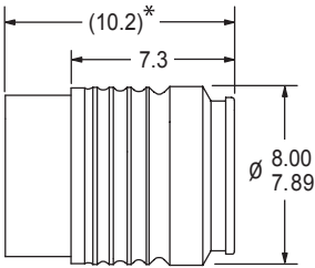
DIMENSIONAL VIEW
