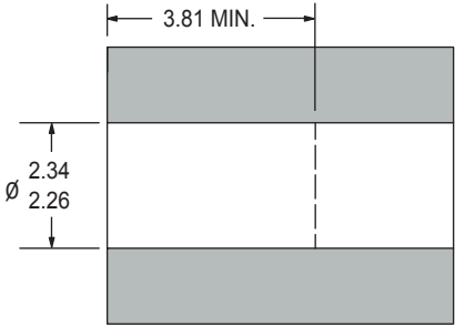
INSTALLATION HOLE
