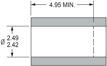
INSTALLATION HOLE
