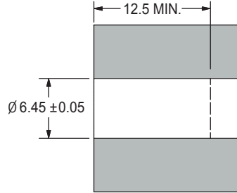
INSTALLATION HOLE
