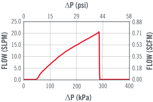
TYPICAL FLOW CURVE for CCVF5530290S
