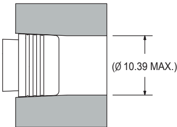
MAXIMUM PASSAGEWAY DIAMETER
