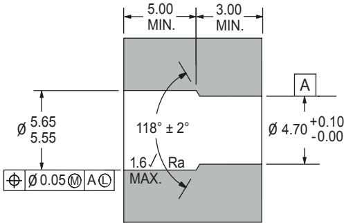
INSTALLATION HOLE
