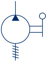
HAND PUMP
