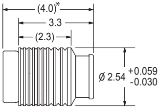
DIMENSIONAL VIEW
