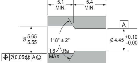
INSTALLATION HOLE
