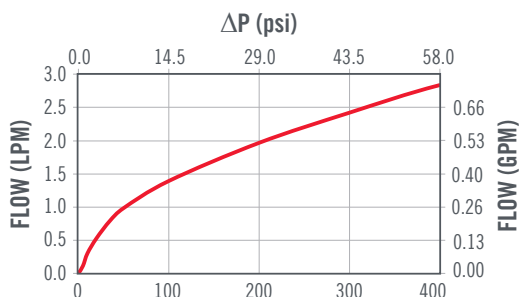
ΔP (kPa) FLOW CURVE FOR 0 kPa VALVE
