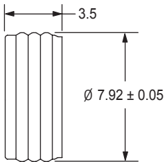
DIMENSIONAL VIEW
