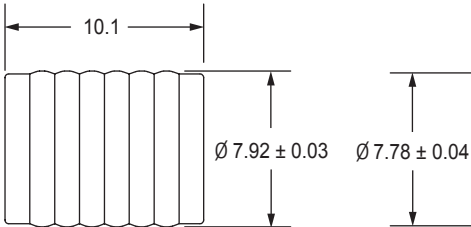
DIMENSIONAL VIEW
