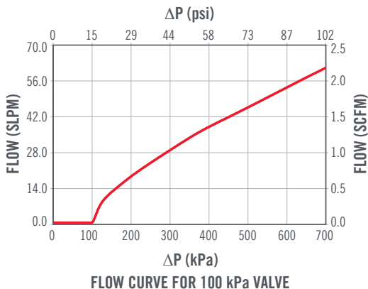
ΔP vs. FLOW ON AIR AT 27°C (80°F)
