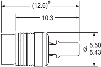
DIMENSIONAL VIEW
