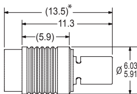
DIMENSIONAL VIEW
