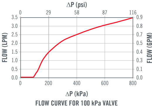
ΔP vs. FLOW ON WATER AT 27°C (80°F)
