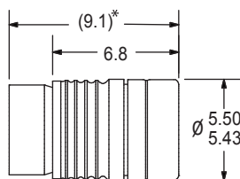
DIMENSIONAL VIEW
