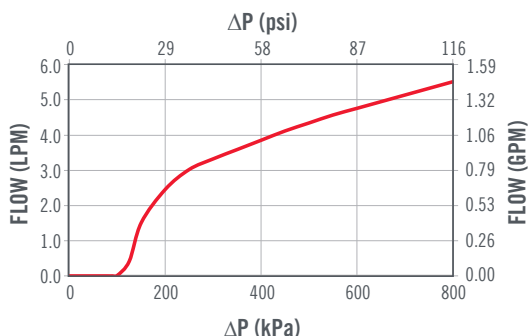
FLOW CURVE FOR 100 kPa VALVE
