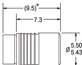
DIMENSIONAL VIEW
