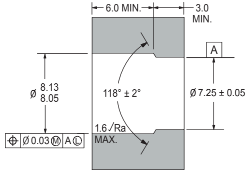
INSTALLATION HOLE
