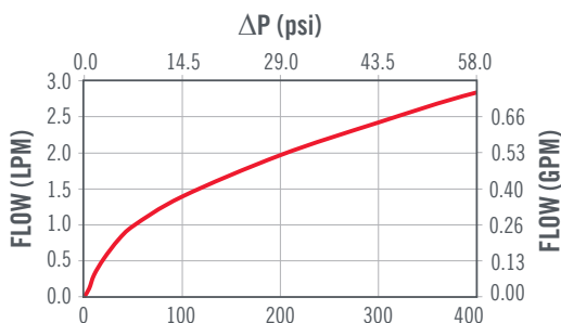
FLOW CURVE FOR 0 kPa VALVE
