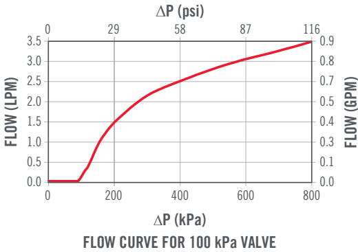
FLOW CURVE FOR 100 kPa VALVE
