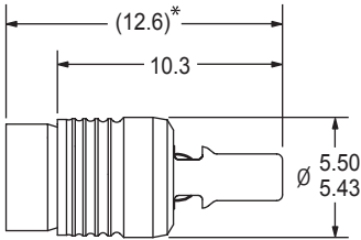
DIMENSIONAL VIEW
