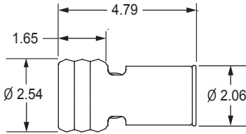
DIMENSIONAL VIEW
