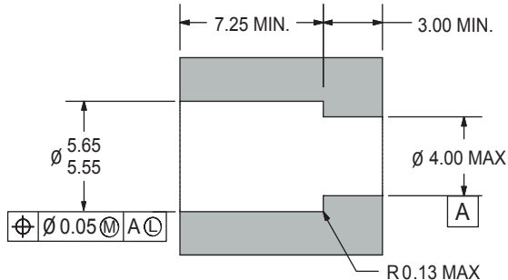
INSTALLATION HOLE
