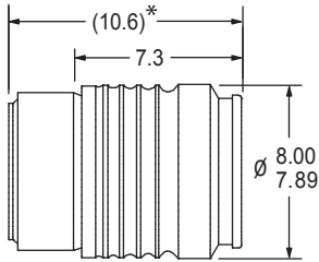
DIMENSIONAL VIEW
