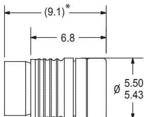
DIMENSIONAL VIEW
