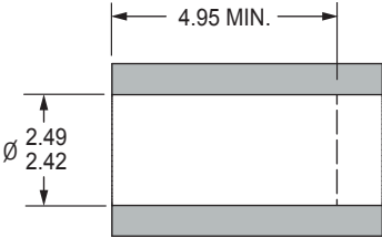
INSTALLATION HOLE
