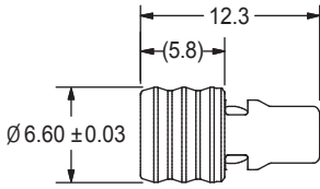
DIMENSIONAL VIEW
