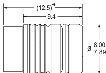
DIMENSIONAL VIEW
