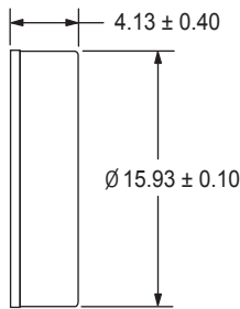
DIMENSIONAL VIEW
