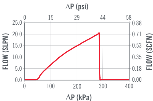
TYPICAL FLOW CURVE for CCVR5530290S
