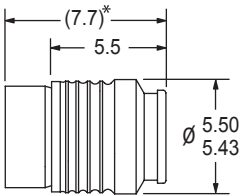
DIMENSIONAL VIEW
