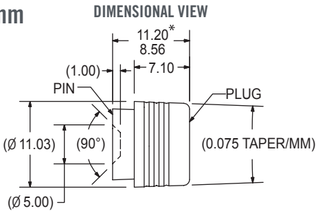
MAXIMUM PASSAGEWAY DIAMETER
