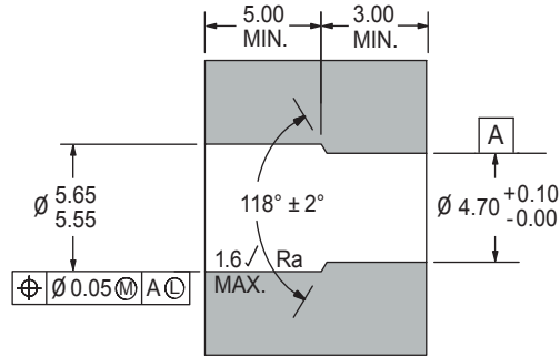
INSTALLATION HOLE
