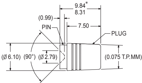
DIMENSIONAL VIEW
