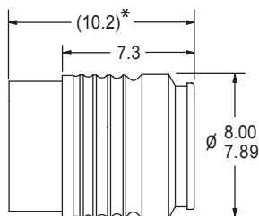
DIMENSIONAL VIEW
