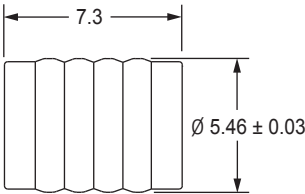
DIMENSIONAL VIEW
