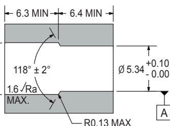
INSTALLATION HOLE
