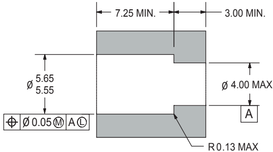
INSTALLATION HOLE
