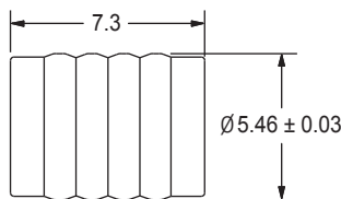
DIMENSIONAL VIEW
