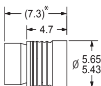
DIMENSIONAL VIEW
