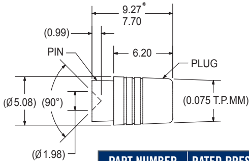
DIMENSIONAL VIEW
