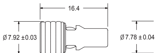
DIMENSIONAL VIEW
