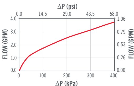
FLOW CURVE FOR 0 kPa VALVE
