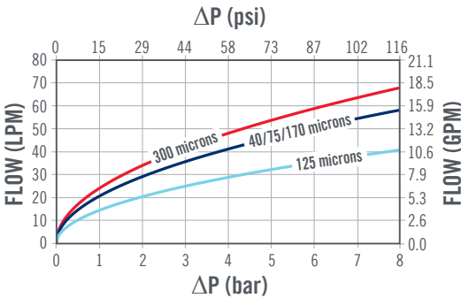
ΔP vs. FLOW ON WATER AT 27°C (80°F)
