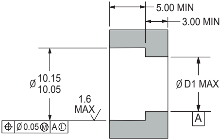
INSTALLATION HOLE
