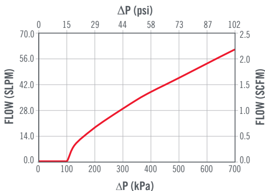
FLOW CURVE FOR 100 kPa VALVE
