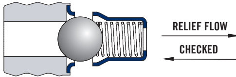
ΔP vs. FLOW ON WATER AT 27°C (80°F)
