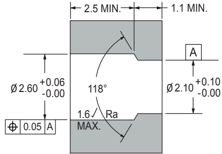
INSTALLATION HOLE
