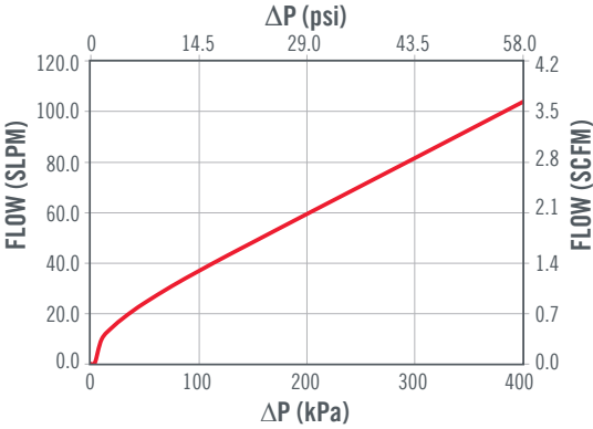
FLOW CURVE FOR 4 kPa VALVE
