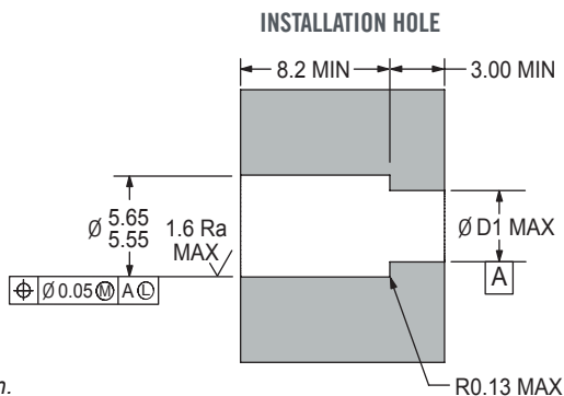
DIMENSIONAL VIEW
