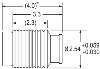
DIMENSIONAL VIEW
