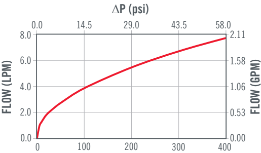
FLOW CURVE FOR 0 kPa VALVE
