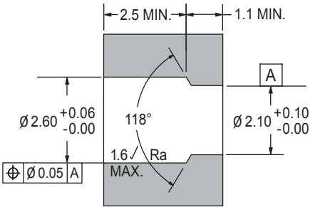
INSTALLATION HOLE
