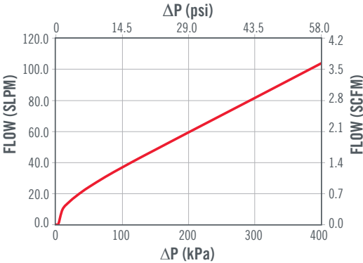
FLOW CURVE FOR 4 kPa VALVE
