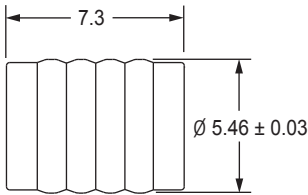
DIMENSIONAL VIEW
