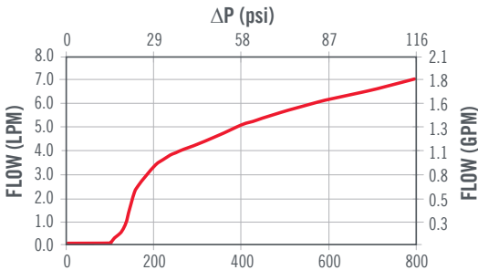
FLOW CURVE FOR 100 kPa VALVE
