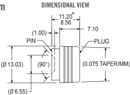
MAXIMUM PASSAGEWAY DIAMETER
