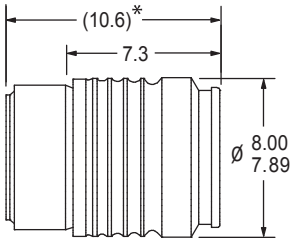
DIMENSIONAL VIEW
