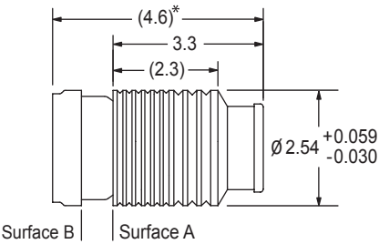
DIMENSIONAL VIEW
