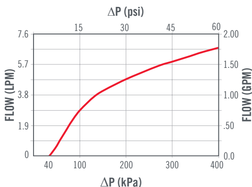
FLOW CURVE FOR 40 kPa VALVE
