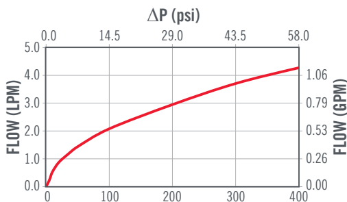
ΔP (kPa) FLOW CURVE FOR 0 kPa VALVE
